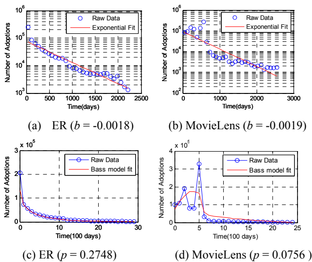
Figure 7: The Distributions of global diffusion time on ER and MovieLens datasets
