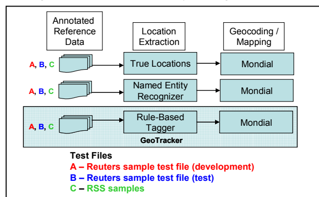
Figure 14 - Experiments framework
